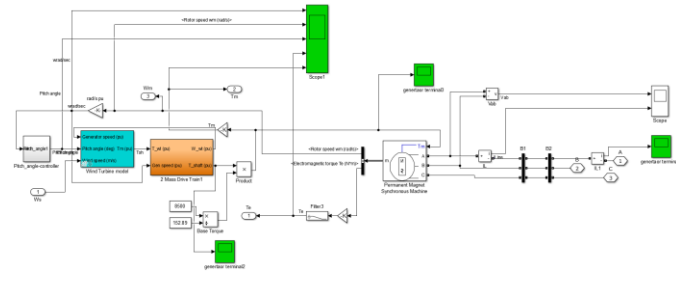
Figure. 13 Wind System MATLAB model diagram
